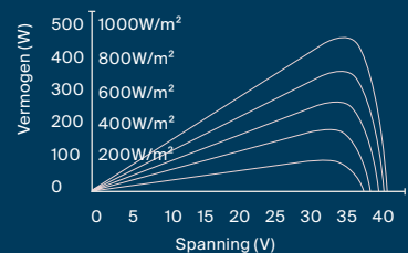
Power-Voltage (420W)
